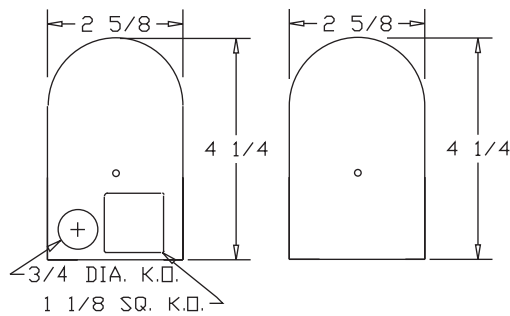
END PLATE
