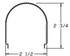
DIFFUSER RIBBED
