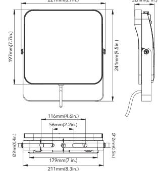
40W&65W(LargeYokeMount)
