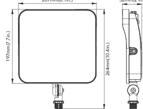
40W&65W(Knuckle Mount)
