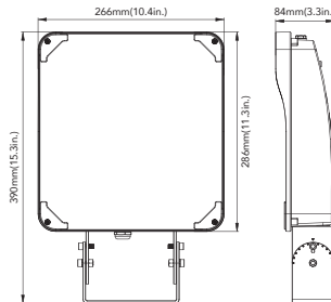
90W&120W(TrunionMount)
