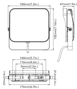
90W&120W(TrunionMount)
