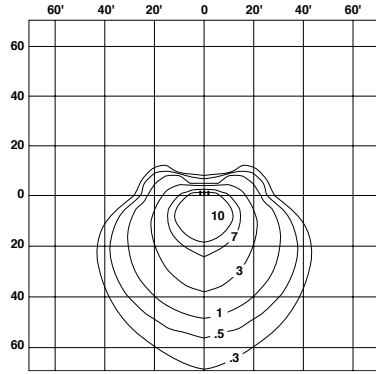
400W MH Wall Pack at 20' mounting height.
